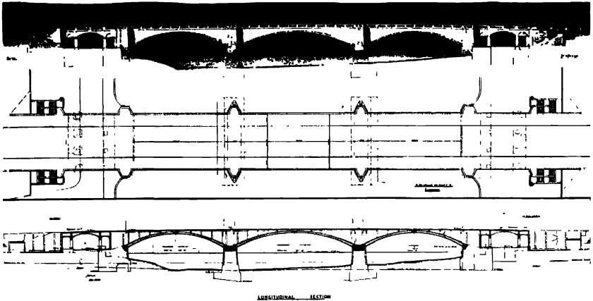
Fig. 358.—Bridge over River Thames at Chiswick.
